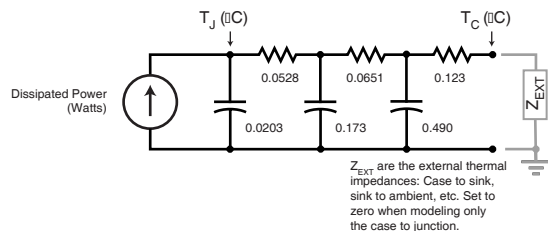
FIGURE 2, TRANSIENT THERMAL IMPEDANCE MODEL
